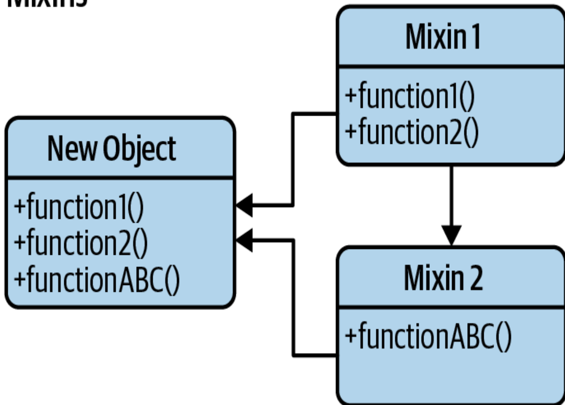
Figure 7-6. Mixins
