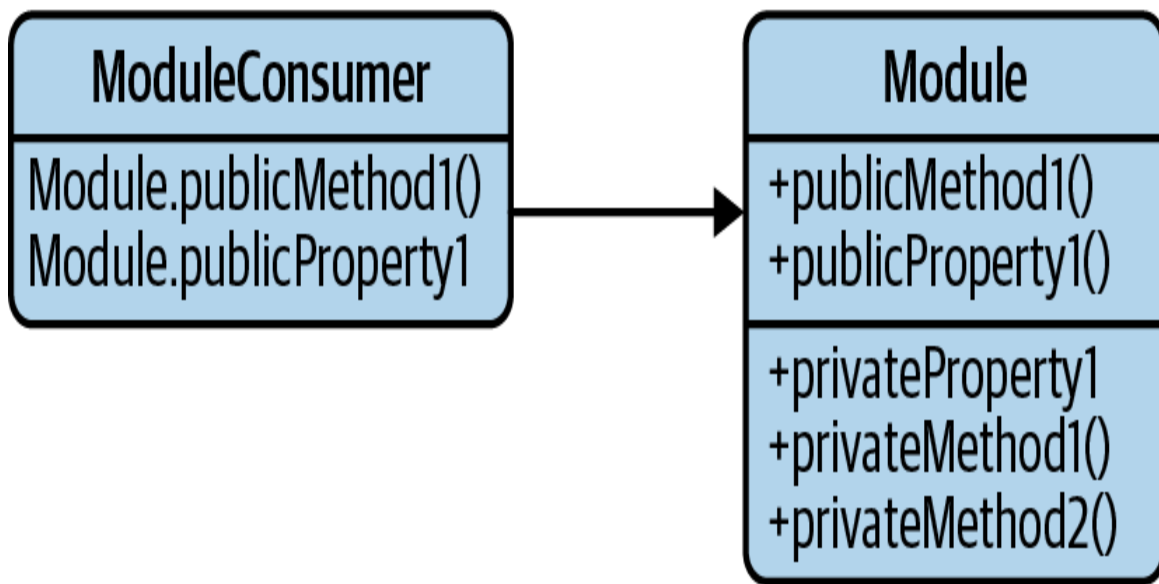
Figure 7-2. Module pattern
