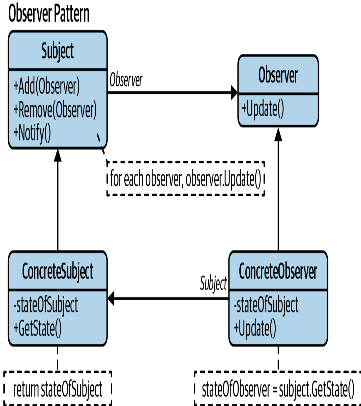
Figure 7-9. Observer pattern
