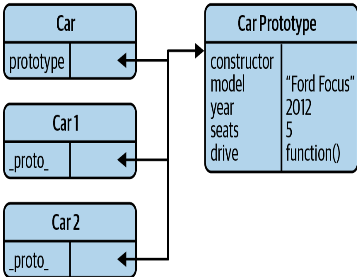
Figure 7-3. Prototype pattern
