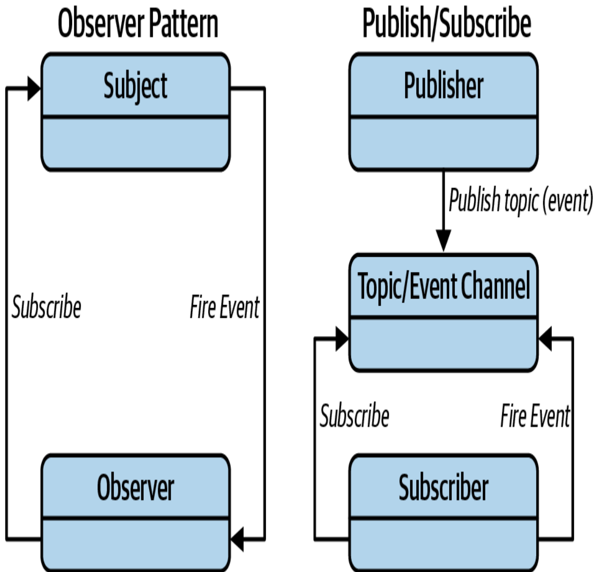
Figure 7-10. Publish/Subscribe
